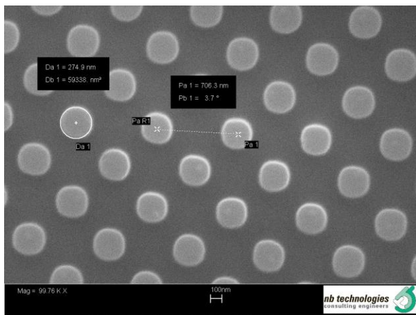
Imprinted dot pattern; dot diameter 275nm/700nm pitch
