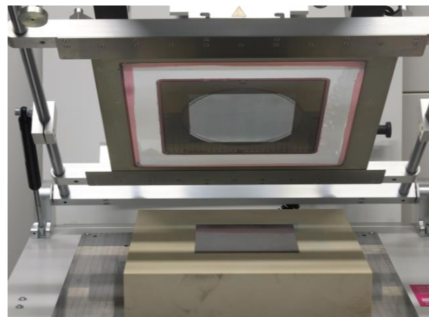
TensoStamp mounted in printing machine
